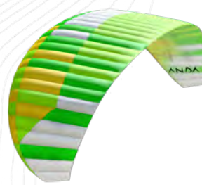
LITHIUM
