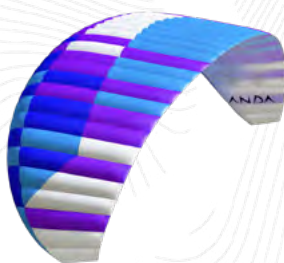
OXYGEN
